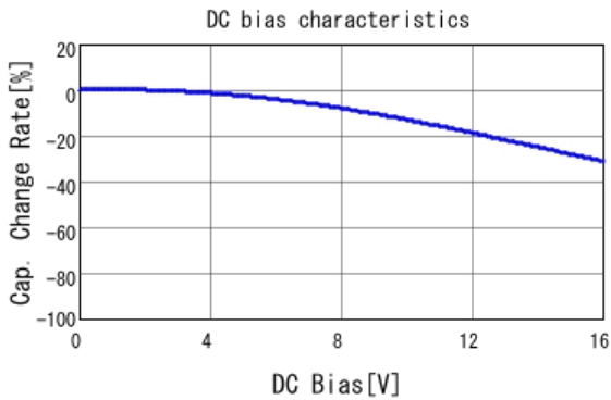
■ GRM319R71C105KAA3 C-DC bias capchange, 25.0degC, AC1.
