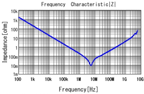
■ GRM319R71C105KAA3 |Z| DCOV, 25degC
