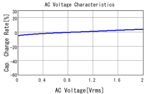
■ GRM319R71C105KAA3 C-AC Voltage capchange, DCOV, 25.0d
