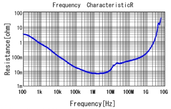
■ GRM319R71C105KAA3 R DCOV, 25degC
