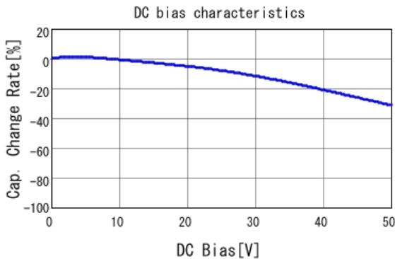
■ GRM319R71H223KA01 C-DC bias capchange, 25.0degC, AC1.
