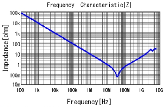
■ GRM319R71H223KA01 |Z| DCOV, 25degC
