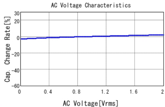
■ GRM319R71H223KA01 C-AC Voltage capchange, DCOV, 25.0d
