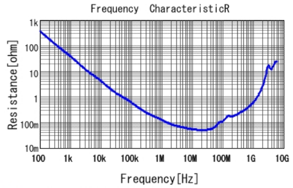
■ GRM319R71H223KA01 R DCOV, 25degC
