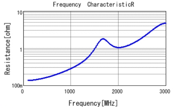
■ GRM31A5C2J101JW01 R DCOV, 25degC
