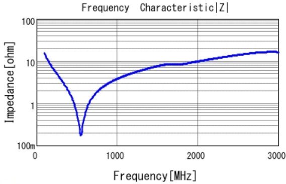
■ GRM31A5C2J101JW01 |Z| DCOV, 25degC
