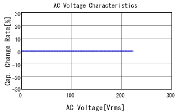
■ GRM31A5C2J101JW01 C-AC Voltage capchange, DCOV, 25.0d
