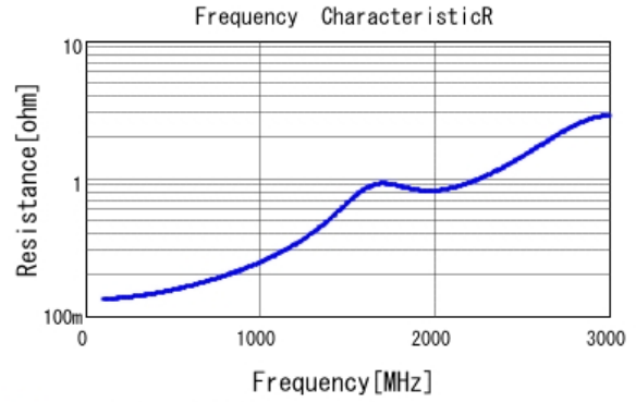
■ GRM31A5C2J151JW01 R DCOV, 25degC
