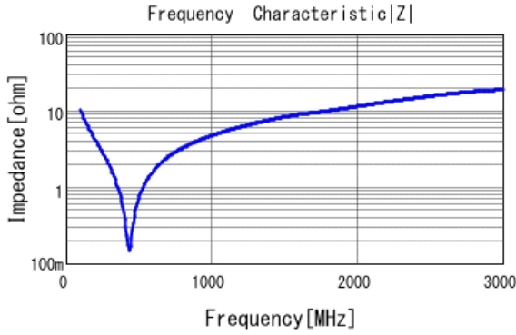
■ GRM31A5C2J151JW01 |Z| DCOV, 25degC
