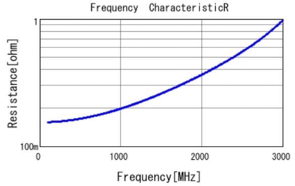
■ GRM31A5C2J220JW01 R DC0V, 25degC
