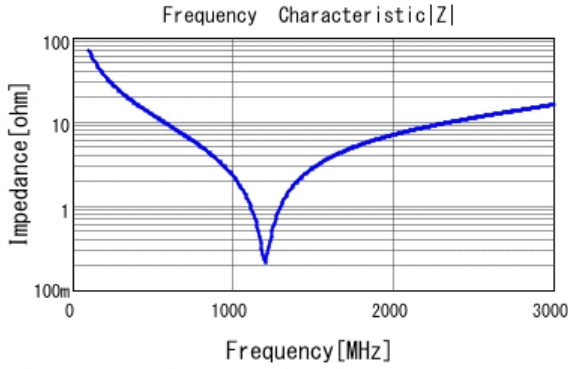
■ GRM31A5C2J220JW01 |Z| DC0V, 25degC
