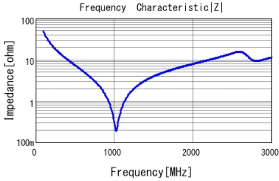
■ GRM31A5C2J330JW01 |Z| DCOV, 25degC
