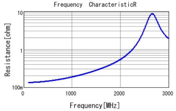
■ GRM31A5C2J330JW01 R DCOV, 25degC
