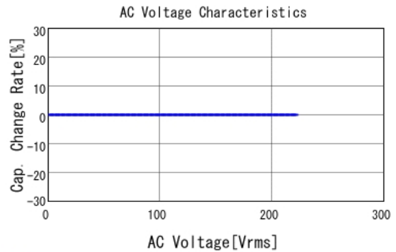
■ GRM31A5C2J330JW01 C-AC Voltage capchange, DCOV, 25.0d
