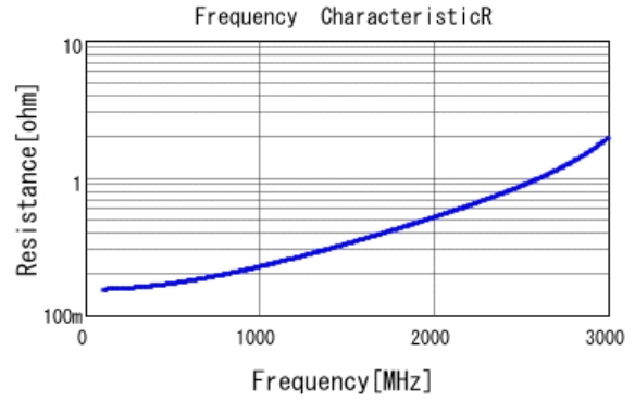
■ GRM31A5C2J470JW01 R DCOV, 25degC
