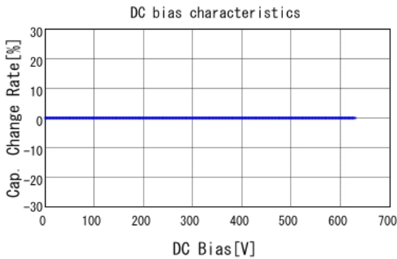
■ GRM31A5C2J470JW01 C-DC bias capchange, 25.0degC, AC1V
