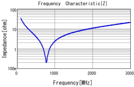
■ GRM31A5C2J470JW01 |Z| DCOV, 25degC
