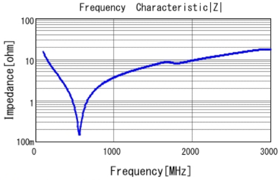
■ GRM31A5C3A101JW01 |Z| DCOV, 25degC
