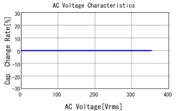
■ GRM31A5C3A101JW01 C-AC Voltage capchange, DCOV, 25.0d
