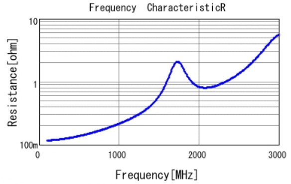
■ GRM31A5C3A101JW01 R DCOV, 25degC
