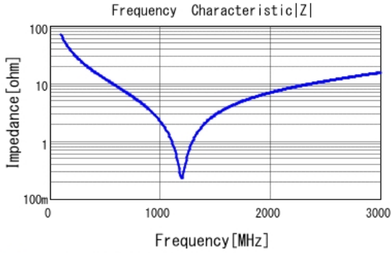
■ GRM31A5C3A220JW01 |Z| DCOV, 25degC
