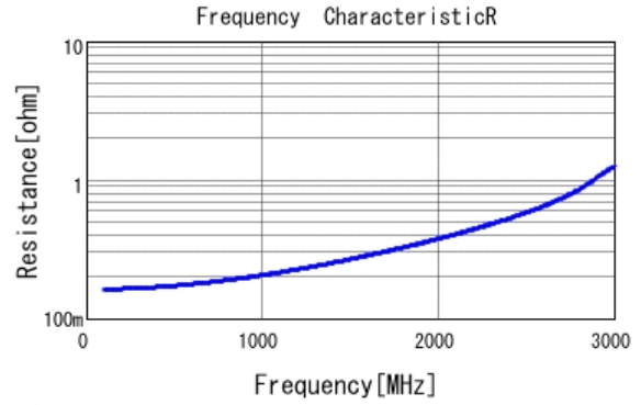
■ GRM31A5C3A220JW01 R DCOV, 25degC
