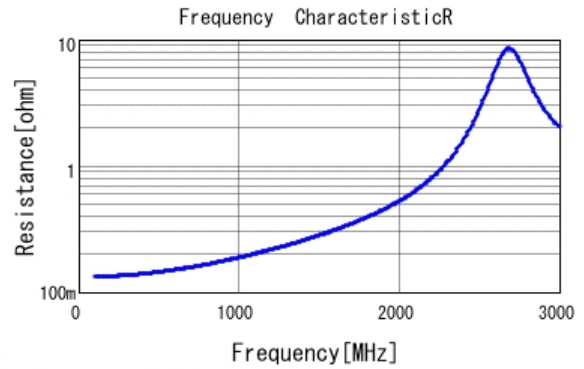
■ GRM31A5C3A330JW01 R DC0V, 25degC
