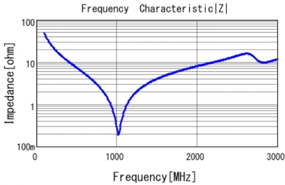
■ GRM31A5C3A330JW01 |Z| DC0V, 25degC
