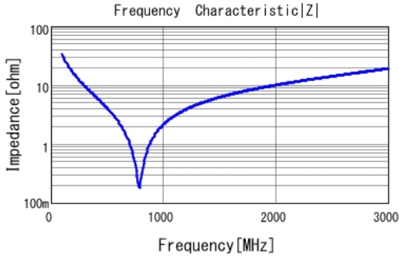
■ GRM31A5C3A470JW01 |Z| DCOV, 25degC
