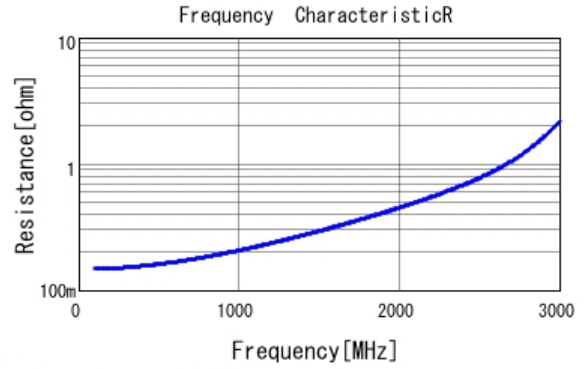
■ GRM31A5C3A470JW01 R DCOV, 25degC
