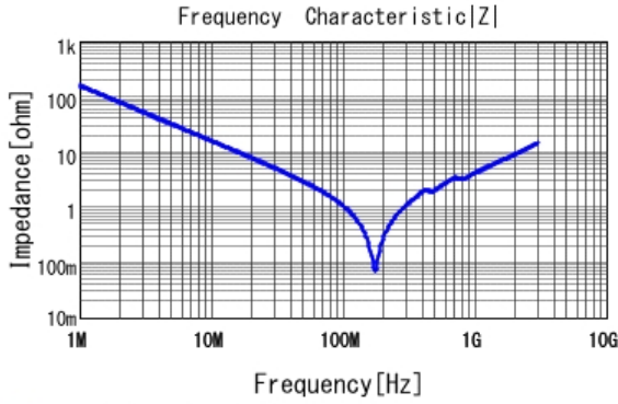
■ GRM31A7U2J102JW31 |Z| DCOV, 25degC
