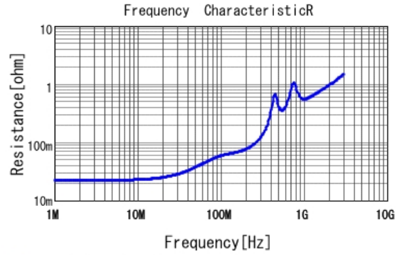
■ GRM31A7U2J102JW31 R DCOV, 25degC
