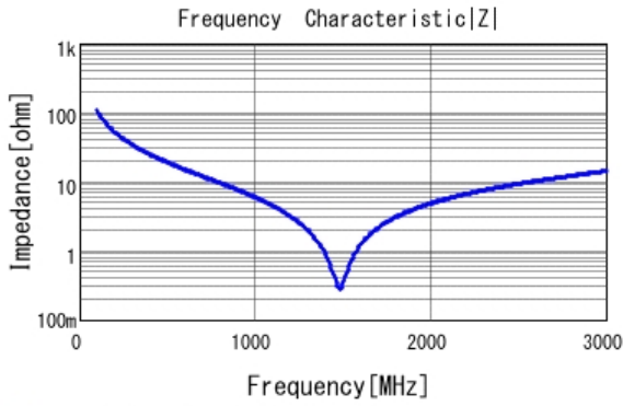
■ GRM31A7U2J150JW31 |Z| DCOV, 25degC
