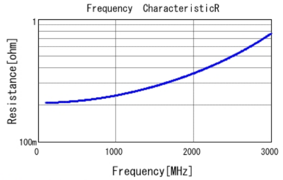
■ GRM31A7U2J150JW31 R DCOV, 25degC
