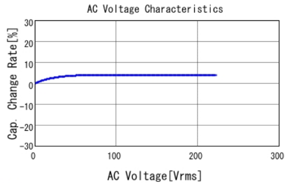
■ GRM31A7U2J150JW31 C-AC Voltage capchange, DCOV, 25.0d
