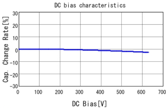
■ GRM31A7U2J152JW31 C-DC bias capchange, 25.0degC, AC1V
