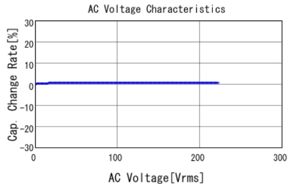
■ GRM31A7U2J152JW31 C-AC Voltage capchange, DCOV, 25.0d
