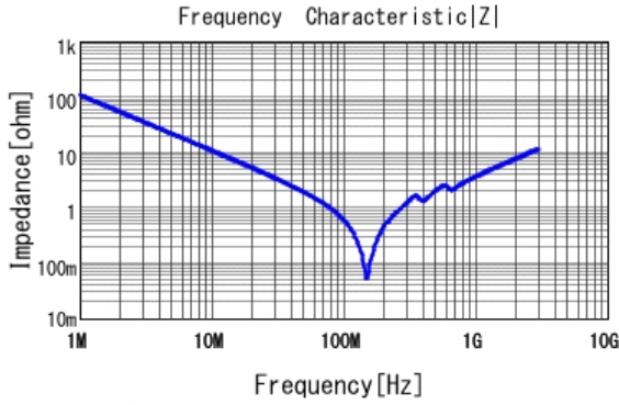
■ GRM31A7U2J152JW31 |Z| DCOV, 25degC
