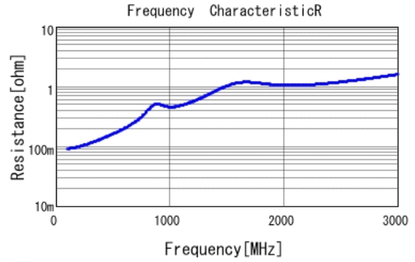
■ GRM31A7U2J471JW31 R DCOV, 25degC
