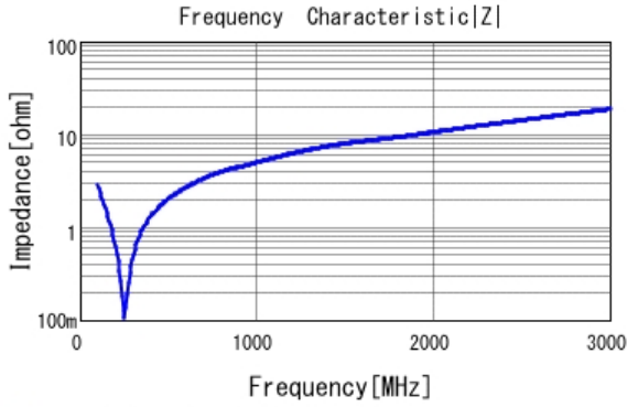
■ GRM31A7U2J471JW31 |Z| DCOV, 25degC
