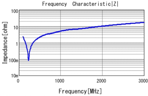
■ GRM31A7U2J561JW31 |Z| DCOV, 25degC
