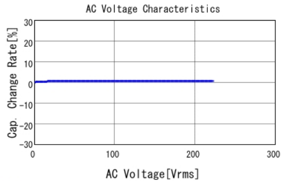
■ GRM31A7U2J561JW31 C-AC Voltage capchange, DCOV, 25.0d
