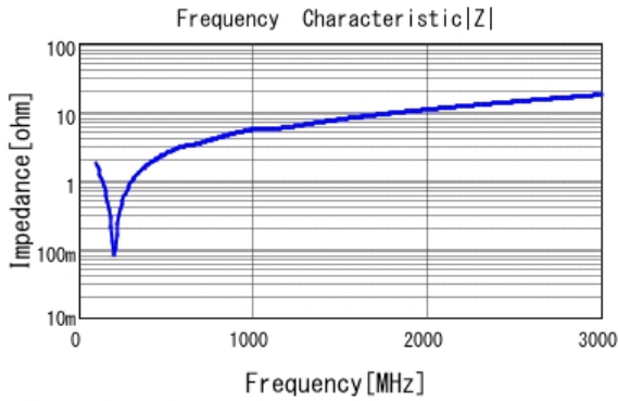
■ GRM31A7U2J681JW31 |Z| DCOV, 25degC
