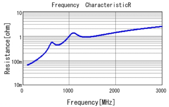
■ GRM31A7U2J681JW31 R DCOV, 25degC
