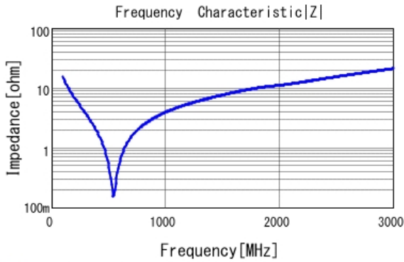
■ GRM31A7U3A101JW31 |Z| DC0V, 25degC
