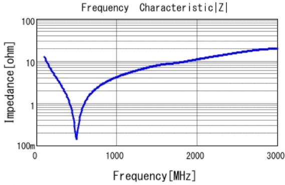
■ GRM31A7U3A121JW31 |Z| DCOV, 25degC
