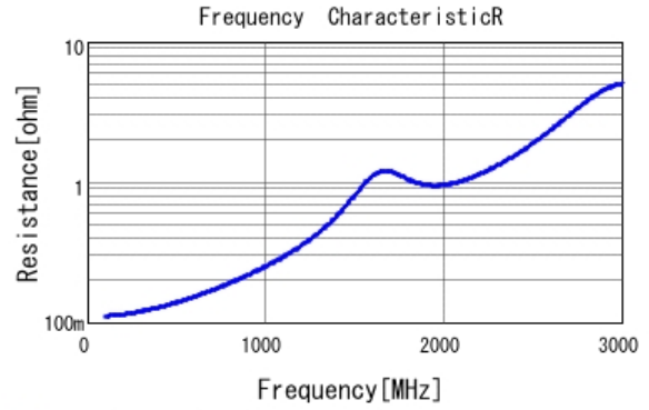
■ GRM31A7U3A121JW31 R DCOV, 25degC
