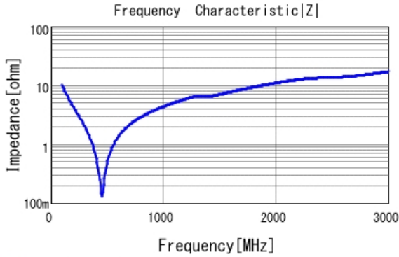
■ GRM31A7U3A151JW31 |Z| DCOV, 25degC
