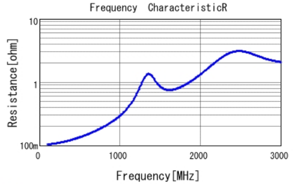
■ GRM31A7U3A151JW31 R DCOV, 25degC
