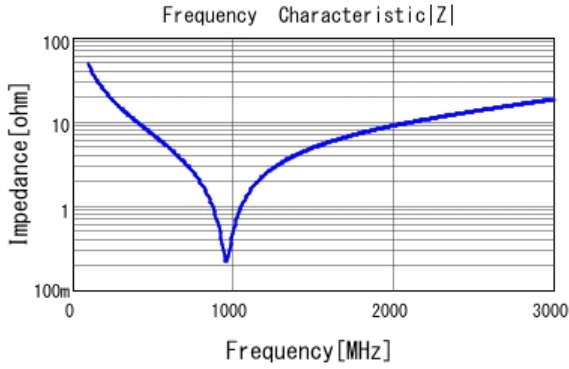
■ GRM31A7U3A330JW31 |Z| DCOV, 25degC
