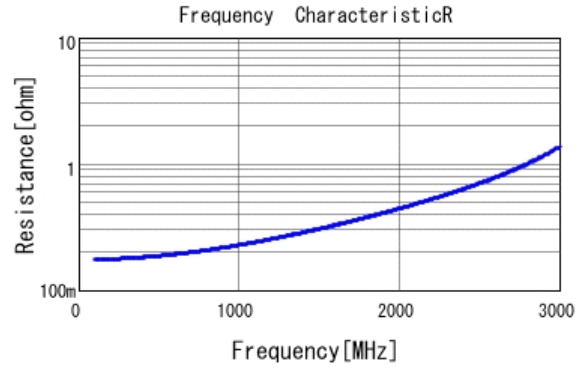
■ GRM31A7U3A330JW31 R DCOV, 25degC
