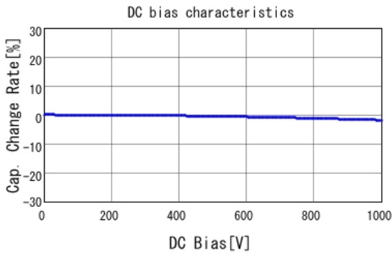
■ GRM31A7U3A330JW31 C-DC bias capchange, 25.0degC, AC1V
