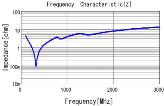
■ GRM31A7U3A331JW31 |Z| DCOV, 25degC
