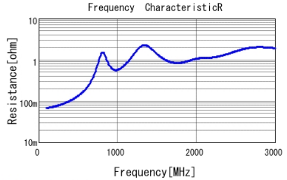
■ GRM31A7U3A331JW31 R DCOV, 25degC
