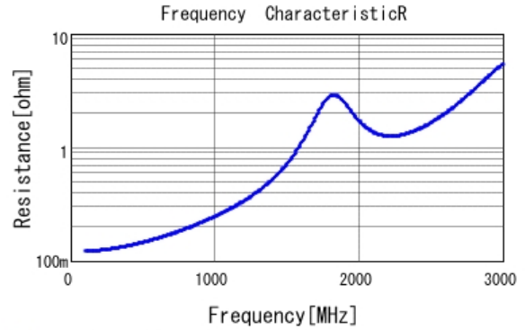
■ GRM31A7U3A680JW31 R DCOV, 25degC
