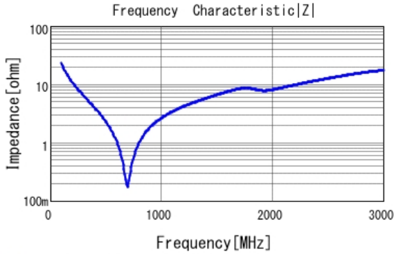
■ GRM31A7U3A680JW31 |Z| DCOV, 25degC
