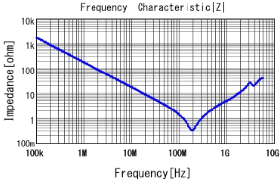
■ GRM31AR72J102KW01 |Z| DCOV, 25degC
