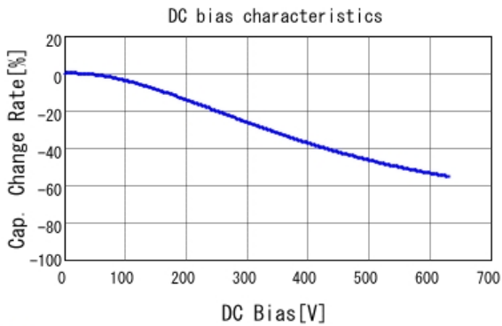
■ GRM31AR72J102KW01 C-DC bias capchange, 25.0degC, AC1V
