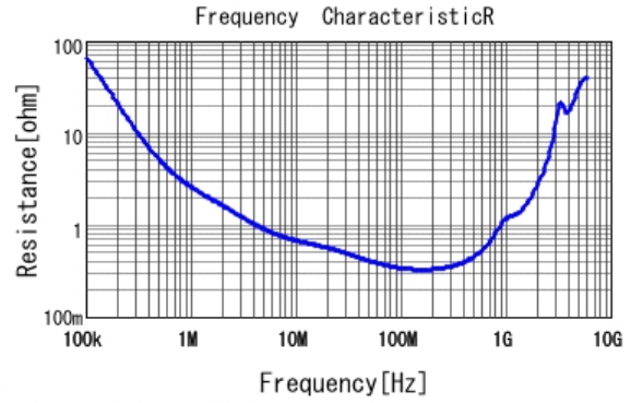
■ GRM31AR72J102KW01 R DCOV, 25degC
