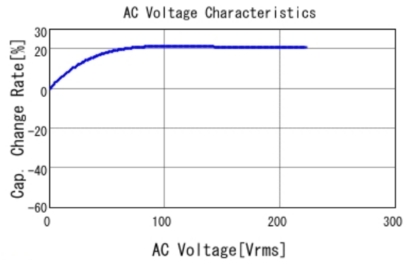
■ GRM31AR72J102KW01 C-AC Voltage capchange, DCOV, 25.0d
