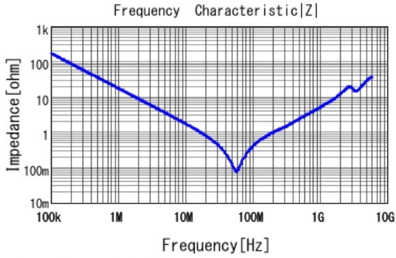
■ GRM31AR72J103KW01 |Z| DCOV, 25degC
