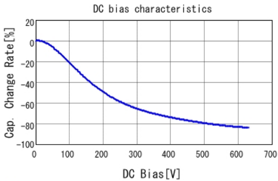
■ GRM31AR72J103KW01 C-DC bias capchange, 25.0degC, AC1V
