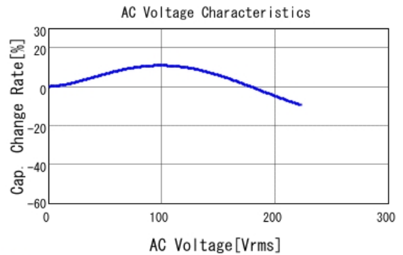
■ GRM31AR72J103KW01 C-AC Voltage capchange, DCOV, 25.0d
