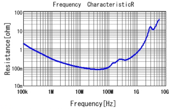
■ GRM31AR72J103KW01 R DCOV, 25degC
