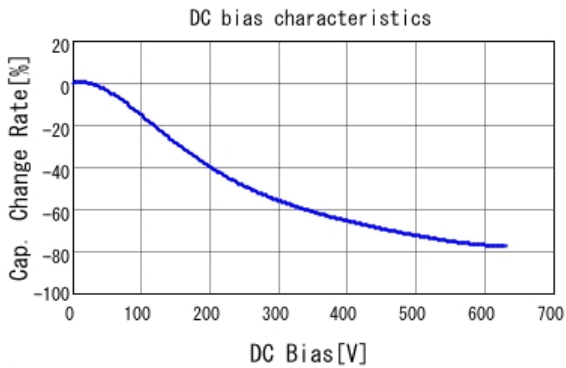
■ GRM31AR72J222KW01 C-DC bias capchange, 25.0degC, AC1V
