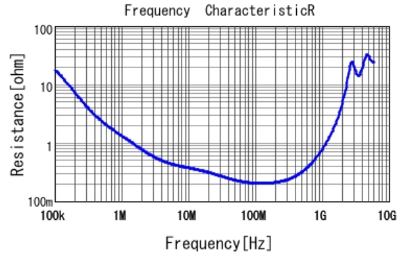
■ GRM31AR72J222KW01 R DCOV, 25degC
