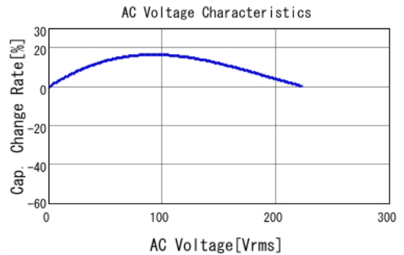
■ GRM31AR72J222KW01 C-AC Voltage capchange, DCOV, 25.0d
