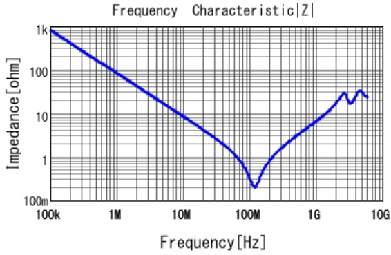
■ GRM31AR72J222KW01 |Z| DCOV, 25degC
