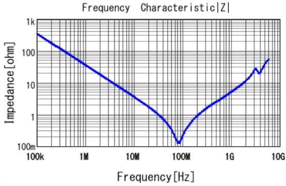
■ GRM31AR72J472KW01 |Z| DCOV, 25degC
