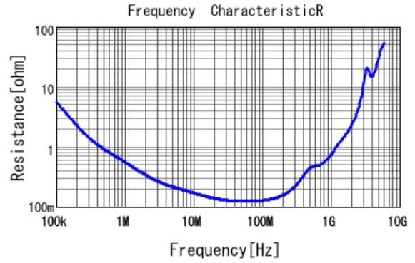
■ GRM31AR72J472KW01 R DCOV, 25degC
