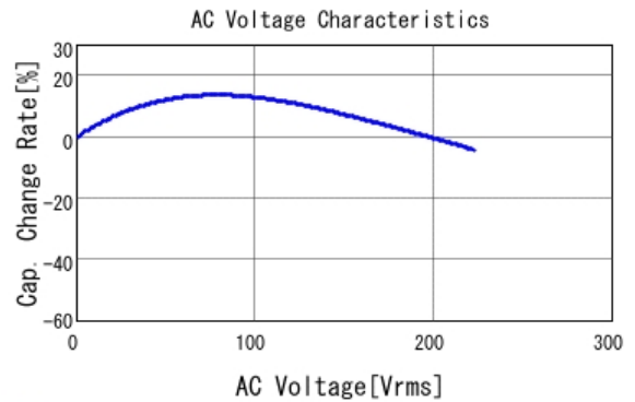
■ GRM31AR72J472KW01 C-AC Voltage capchange, DCOV, 25.0d
