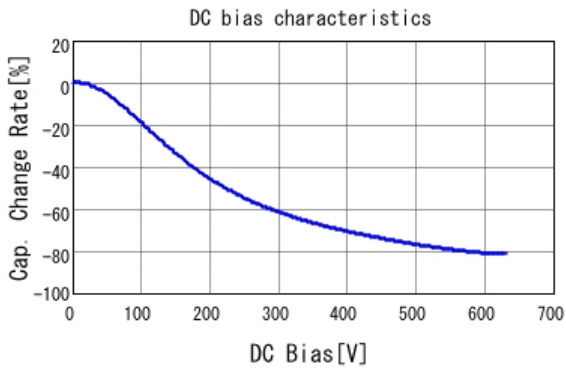
■ GRM31AR72J472KW01 C-DC bias capchange, 25.0degC, AC1V
