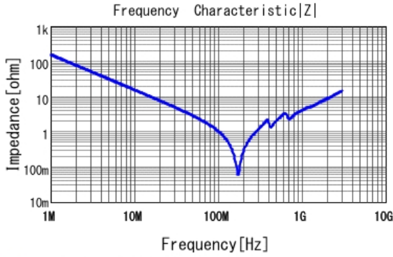
■ GRM31B5C2J102JW01 |Z| DCOV, 25degC
