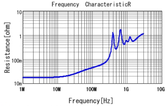
■ GRM31B5C2J102JW01 R DCOV, 25degC
