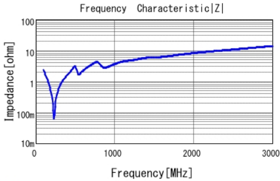
■ GRM31B5C3A561JWA1 |Z| DCOV, 25degC
