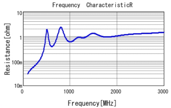
■ GRM31B5C3A561JWA1 R DCOV, 25degC
