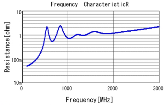
■ GRM31B7U3A471JW31 R DCOV, 25degC
