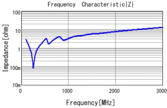
■ GRM31B7U3A471JW31 |Z| DCOV, 25degC
