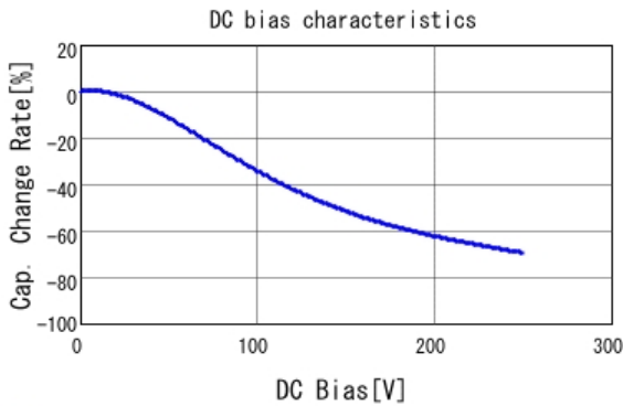
■ GRM31BR72E153KW01 C-DC bias capchange, 25.0degC, AC1V
