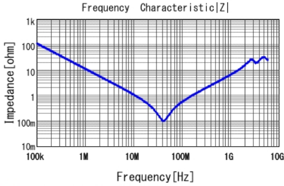
■ GRM31BR72E153KW01 |Z| DCOV, 25degC
