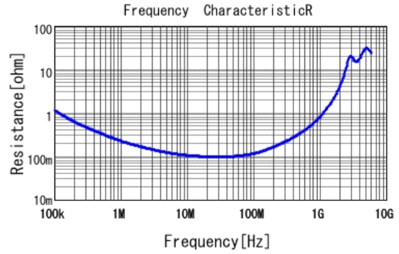
■ GRM31BR72E153KW01 R DCOV, 25degC
