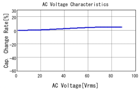
■ GRM31BR72E153KW01 C-AC Voltage capchange, DCOV, 25.0d
