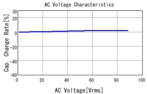
■ GRM31BR72E223KW01 C-AC Voltage capchange, DCOV, 25.0d
