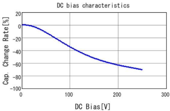
■ GRM31BR72E223KW01 C-DC bias capchange, 25.0degC, AC1V
