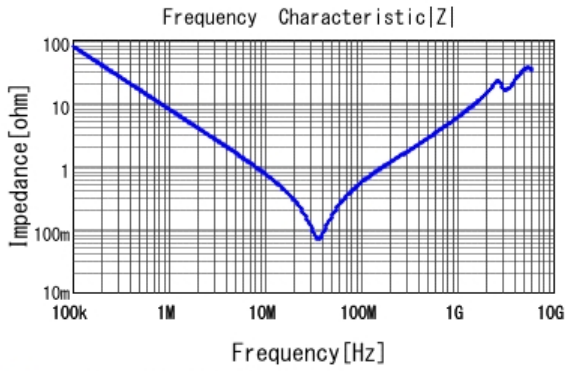
■ GRM31BR72E223KW01 |Z| DCOV, 25degC
