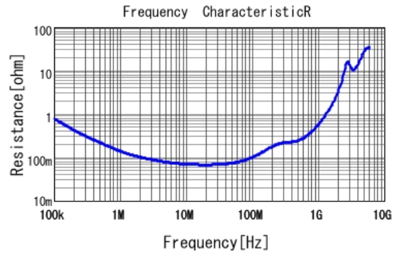
■ GRM31BR72E223KW01 R DCOV, 25degC
