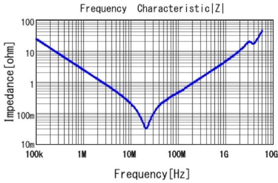
■ GRM31BR72E683KW01 |Z| DCOV, 25degC
