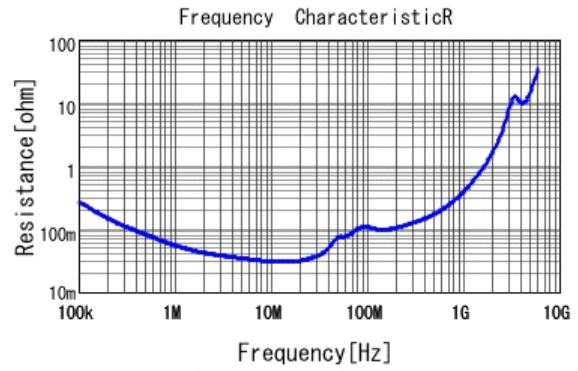
■ GRM31BR72E683KW01 R DCOV, 25degC
