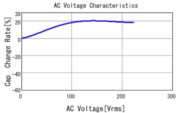
■ GRM31BR72J102KW01 C-AC Voltage capchange, DCOV, 25.0d
