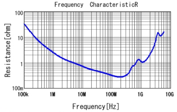
■ GRM31BR72J102KW01 R DCOV, 25degC
