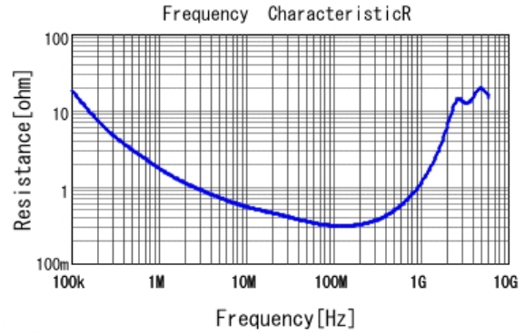
■ GRM31BR72J152KW01 R DCOV, 25degC
