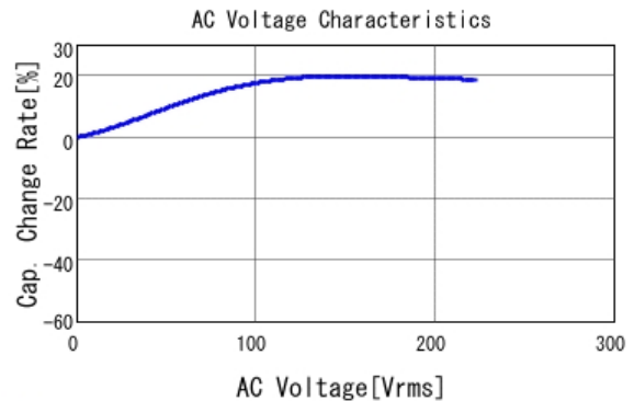
■ GRM31BR72J152KW01 C-AC Voltage capchange, DCOV, 25.0d
