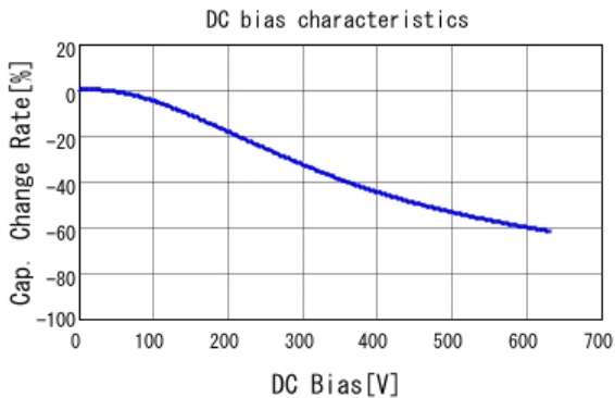
■ GRM31BR72J152KW01 C-DC bias capchange, 25.0degC, AC1V
