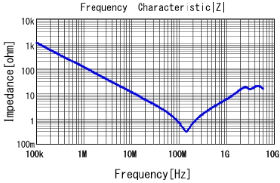
■ GRM31BR72J152KW01 |Z| DCOV, 25degC
