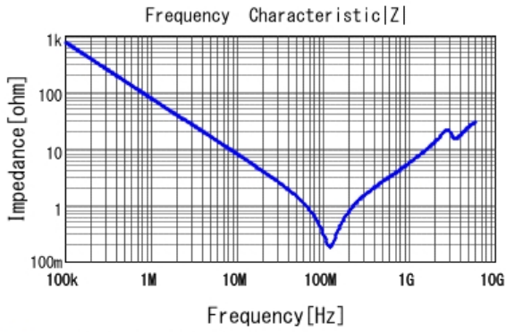
■ GRM31BR72J222KW01 |Z| DCOV, 25degC
