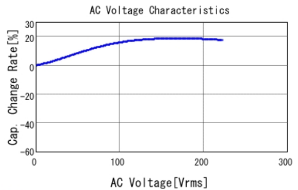
■ GRM31BR72J222KW01 C-AC Voltage capchange, DCOV, 25.0d
