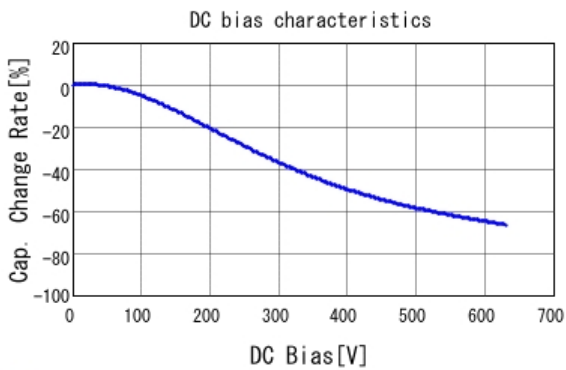
■ GRM31BR72J222KW01 C-DC bias capchange, 25.0degC, AC1V
