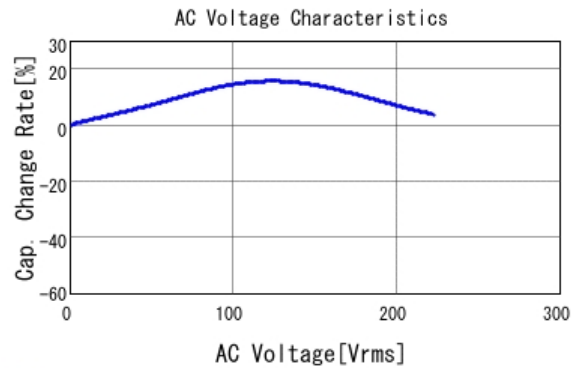
■ GRM31BR72J332KW01 C-AC Voltage capchange, DCOV, 25.0d
