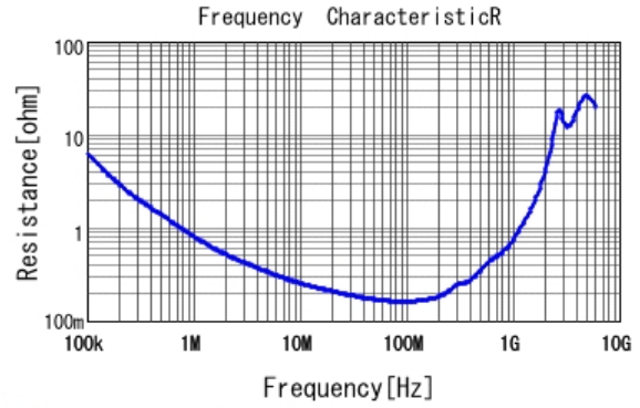
■ GRM31BR72J332KW01 R DCOV, 25degC
