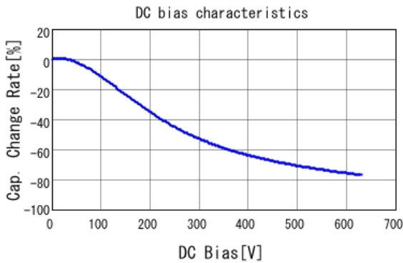
■ GRM31BR72J332KW01 C-DC bias capchange, 25.0degC, AC1V
