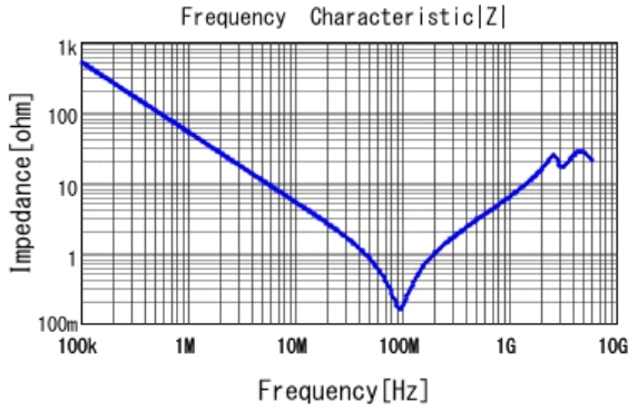
■ GRM31BR72J332KW01 |Z| DCOV, 25degC
