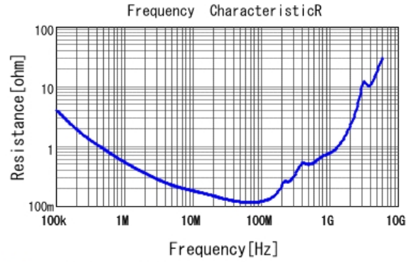
■ GRM31BR72J472KW01 R DCOV, 25degC
