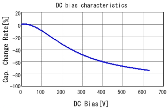
■ GRM31BR72J472KW01 C-DC bias capchange, 25.0degC, AC1V
