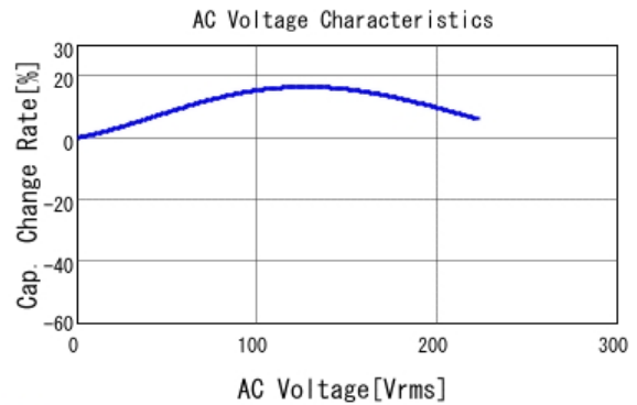
■ GRM31BR72J472KW01 C-AC Voltage capchange, DCOV, 25.0d
