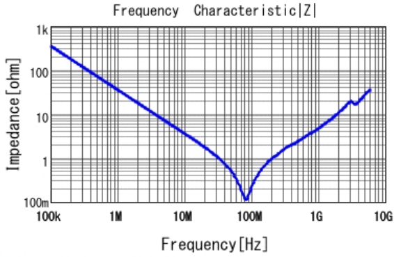
■ GRM31BR72J472KW01 |Z| DCOV, 25degC
