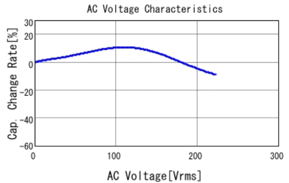
■ GRM31BR72J682KW01 C-AC Voltage capchange, DCOV, 25.0d
