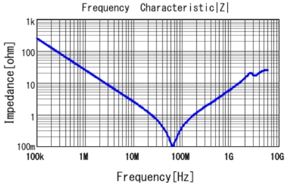
■ GRM31BR72J682KW01 |Z| DCOV, 25degC
