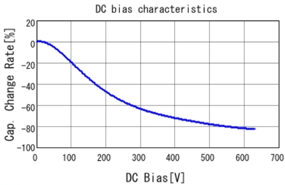
■ GRM31BR72J682KW01 C-DC bias capchange, 25.0degC, AC1V
