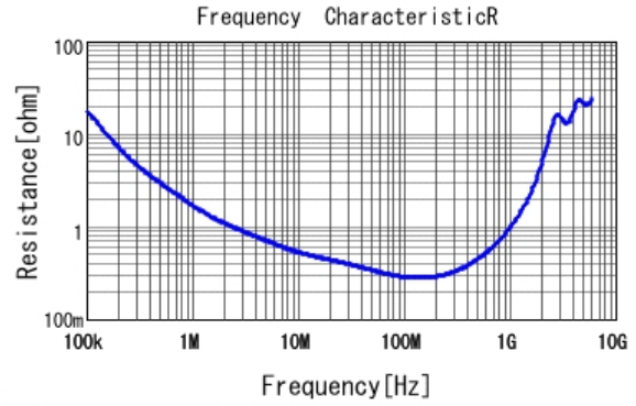
■ GRM31BR73A152KW01 R DCOV, 25degC
