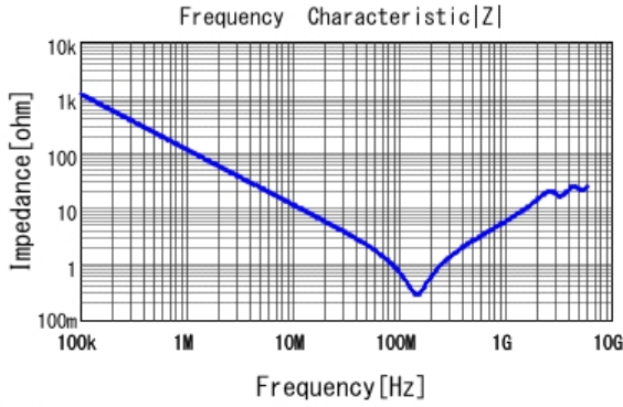
■ GRM31BR73A152KW01 |Z| DCOV, 25degC
