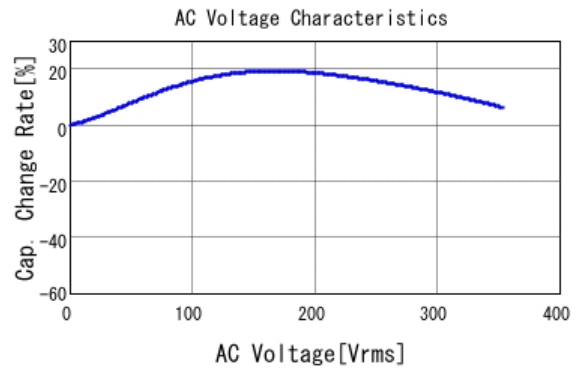
■ GRM31BR73A152KW01 C-AC Voltage capchange, DCOV, 25.0d
