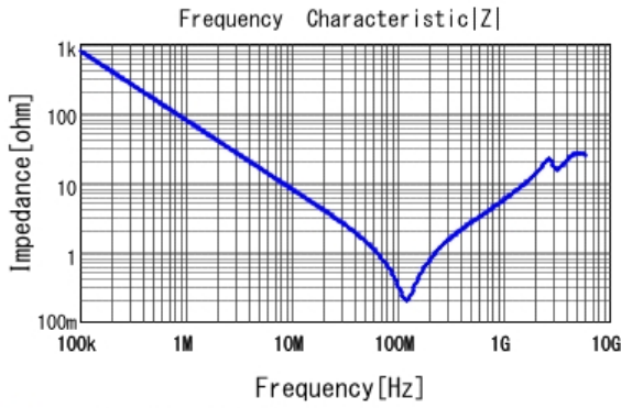
■ GRM31BR73A222KW01 |Z| DCOV, 25degC
