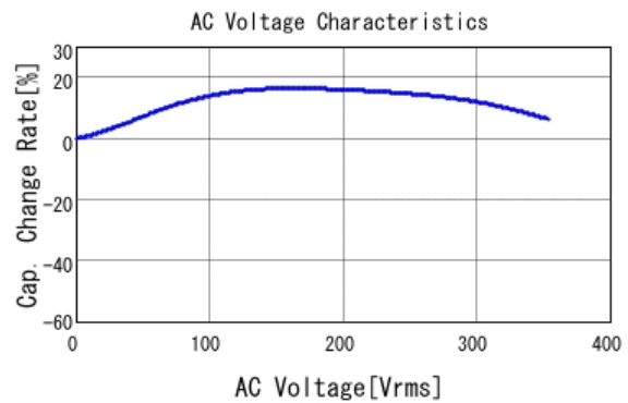
■ GRM31BR73A222KW01 C-AC Voltage capchange, DCOV, 25.0d
