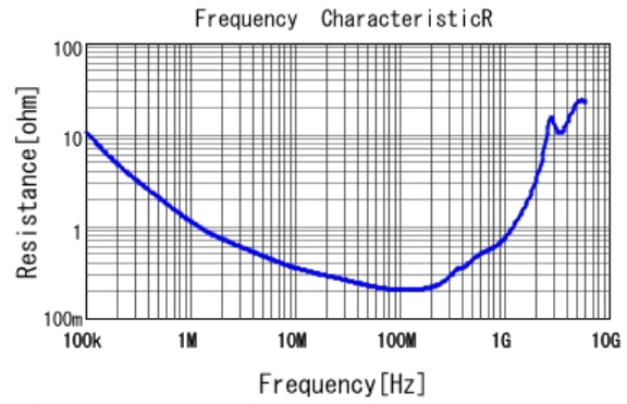
■ GRM31BR73A222KW01 R DCOV, 25degC
