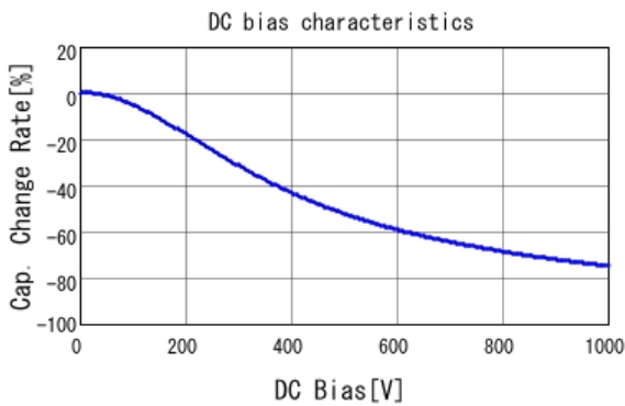
■ GRM31BR73A222KW01 C-DC bias capchange, 25.0degC, AC1V
