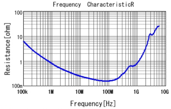
■ GRM31BR73A332KW01 R DCOV, 25degC
