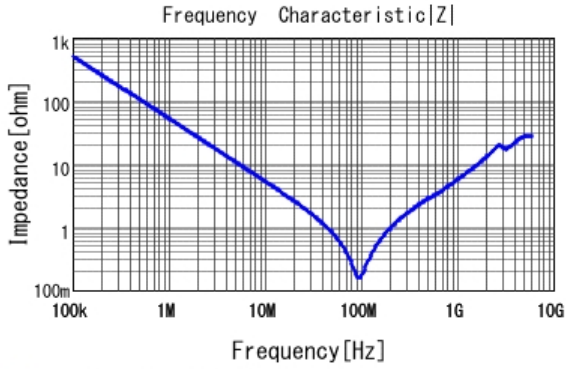
■ GRM31BR73A332KW01 |Z| DCOV, 25degC
