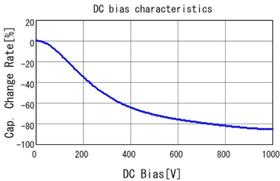
■ GRM31BR73A332KW01 C-DC bias capchange, 25.0degC, AC1V
