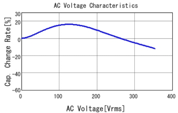
■ GRM31BR73A332KW01 C-AC Voltage capchange, DCOV, 25.0d
