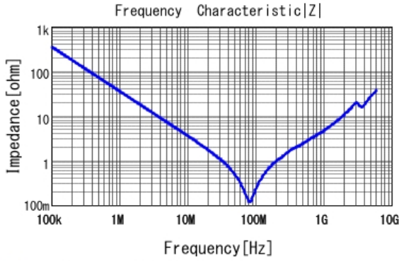
■ GRM31BR73A472KW01 |Z| DCOV, 25degC
