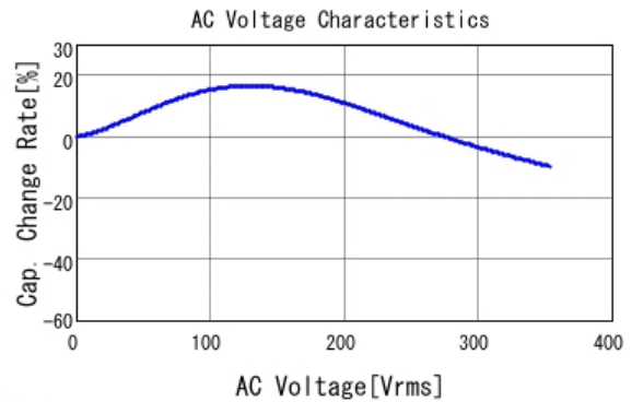
■ GRM31BR73A472KW01 C-AC Voltage capchange, DCOV, 25.0d
