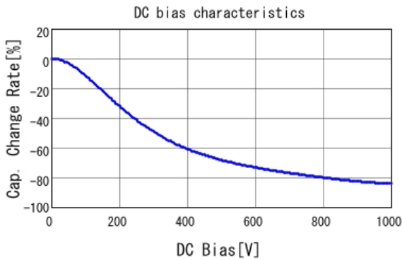
■ GRM31BR73A472KW01 C-DC bias capchange, 25.0degC, AC1V
