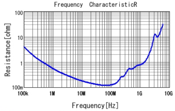
■ GRM31BR73A472KW01 R DCOV, 25degC
