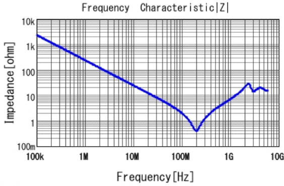
■ GRM31BR73A681KW01 |Z| DCOV, 25degC
