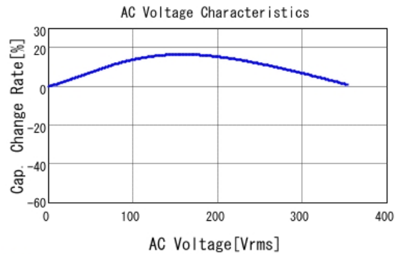
■ GRM31BR73A681KW01 C-AC Voltage capchange, DCOV, 25.0d
