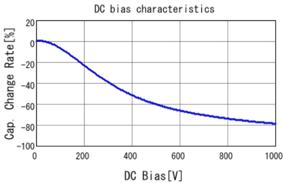
■ GRM31BR73A681KW01 C-DC bias capchange, 25.0degC, AC1V
