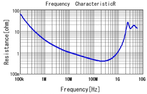
■ GRM31BR73A681KW01 R DCOV, 25degC
