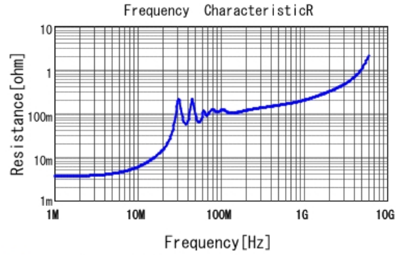
■ GRM31C5C1H104JA01 R DC0V, 25degC
