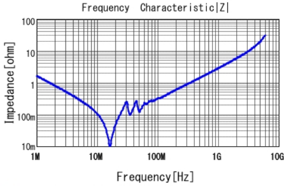
■ GRM31C5C1H104JA01 |Z| DC0V, 25degC
