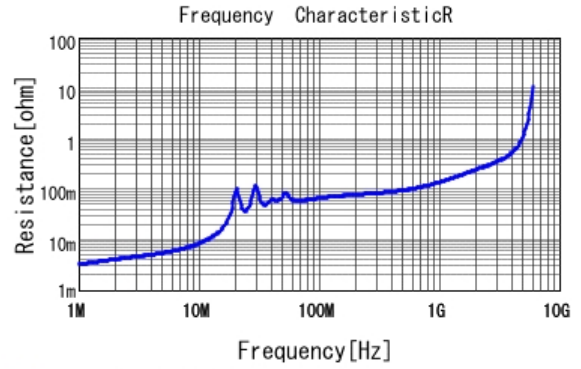
■ GRM31C5C1H224JE02 R DCOV, 25degC
