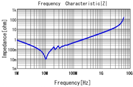
■ GRM31C5C1H224JE02 |Z| DCOV, 25degC
