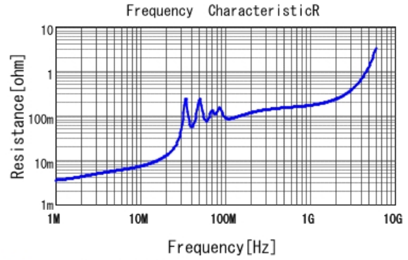
■ GRM31C5C1H823JA01 R DCOV, 25degC
