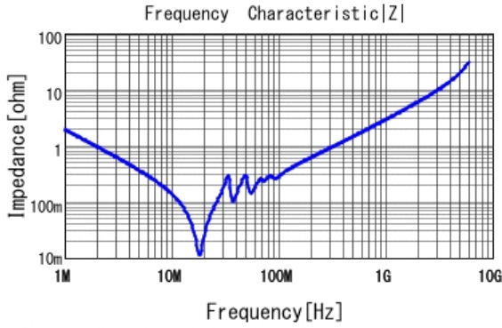
■ GRM31C5C1H823JA01 |Z| DCOV, 25degC
