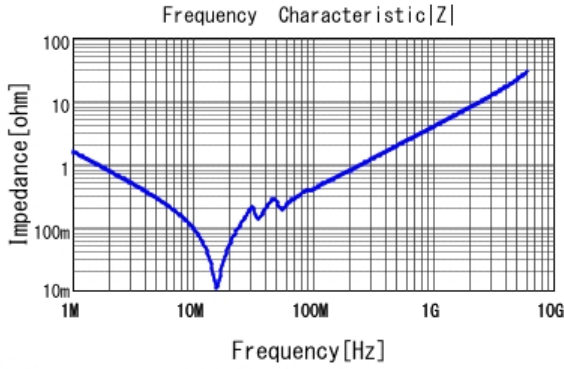
■ GRM31C5C2A104JA01 |Z| DCOV, 25degC
