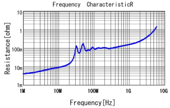
■ GRM31C5C2A104JA01 R DCOV, 25degC
