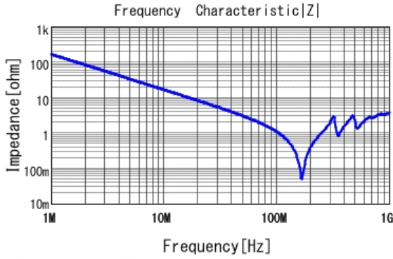
■ GRM31C5C3A102JWA3 |Z| DCOV, 25degC
