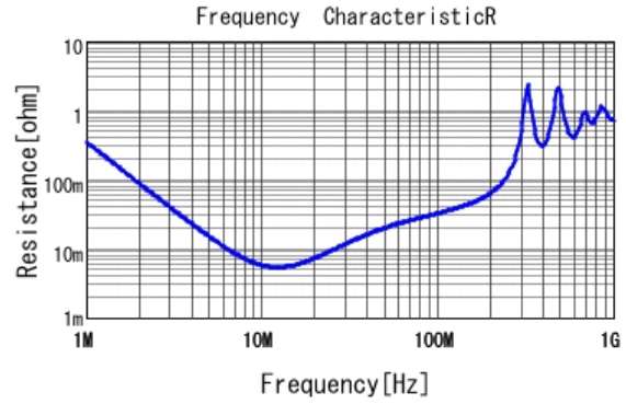
■ GRM31C5C3A102JWA3 R DCOV, 25degC
