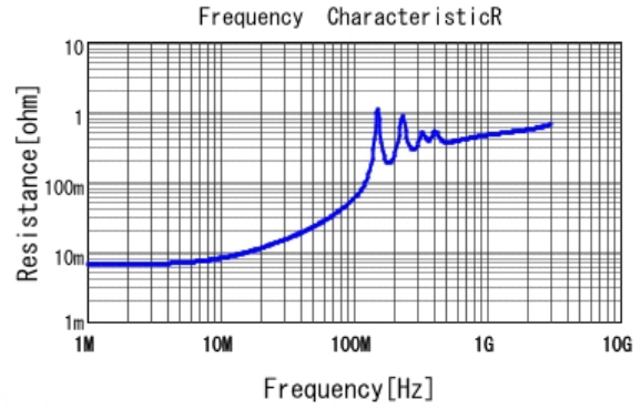
■ GRM31C7U2J472JW32 R DCOV, 25degC
