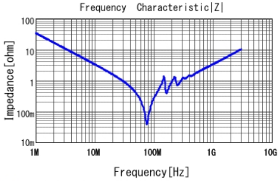
■ GRM31C7U2J472JW32 |Z| DCOV, 25degC
